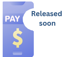
Payment Gateway
